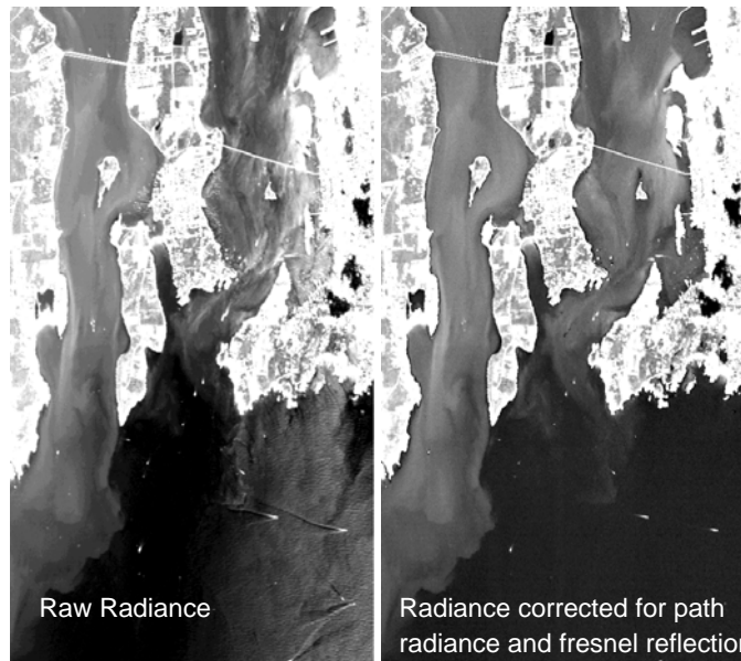
Figure 3. Example of Removal of Pixel Dependent Path Radiance and Fresnel Reflections for the 580 nm Band.
