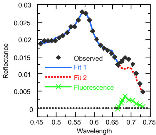
Figure 6b. Example solutions of the fit of the model equation to two AVIRIS spectra. The plot on the left shows a low phytoplankton, low fluorescence solution, while the plot on the right shows a high phytoplankton, high fluorescence solution.
