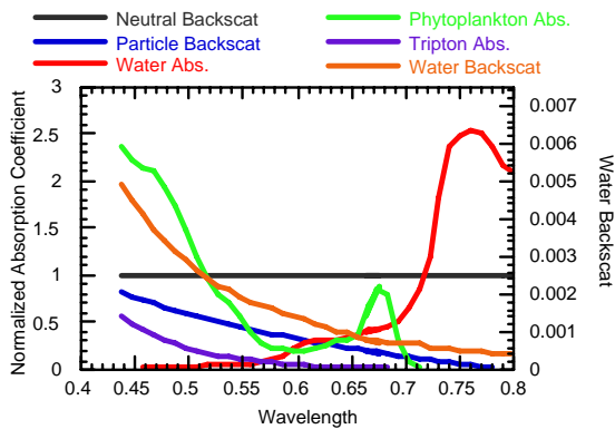
Figure 5. Basis Vectors for Absorption and Scattering Components.
