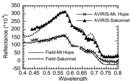
Figure 4. Comparison Between AVIRIS Apparent Reflectance Spectra and Field Spectra Acquired with an ASD FieldSpec FR.
