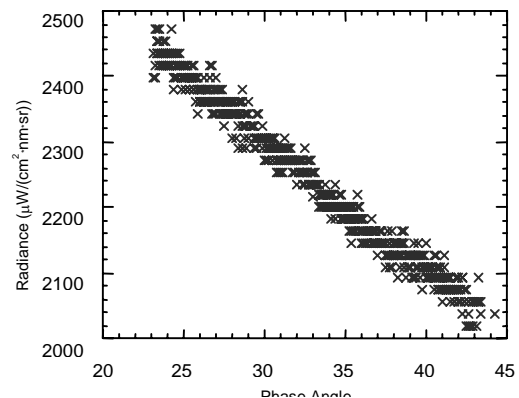
Figure 2. Phase Angle Dependence of Path Radiance.
